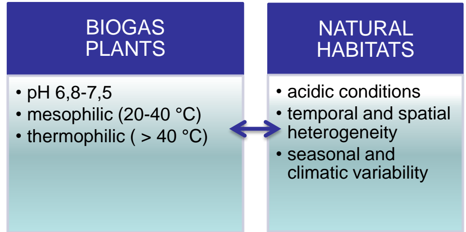
Fig. 2: Comparison of biogas plants and natural habitats
